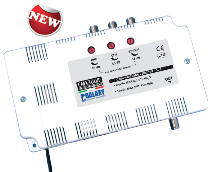
★ CENTRALINI DA INTERNO SERIE "CMX" ... AMPLIFIERS FOR INDOOR USE "CMX" SERIES ...
