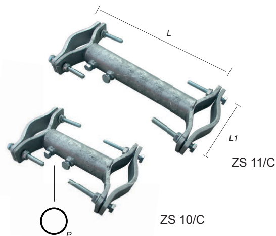
ZANCHE TELESCOPICHE PALO/PALO . . . MAST/MAST TELESCOPIC BRACKETS . . .
