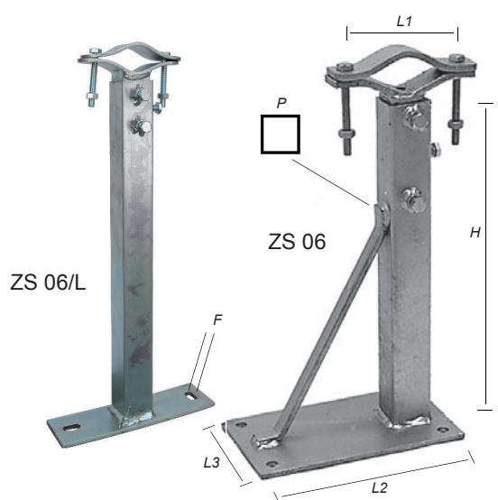
ZANCHE TELESCOPICHE PALO/MURO . . . TELESCOPIC MAST/WALL BRACKETS . . .
