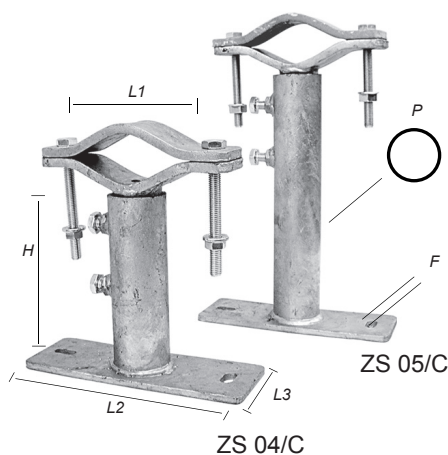
ZANCHE TELESCOPICHE PALO/MURO . . . TELESCOPIC MAST/WALL BRACKETS . . .
